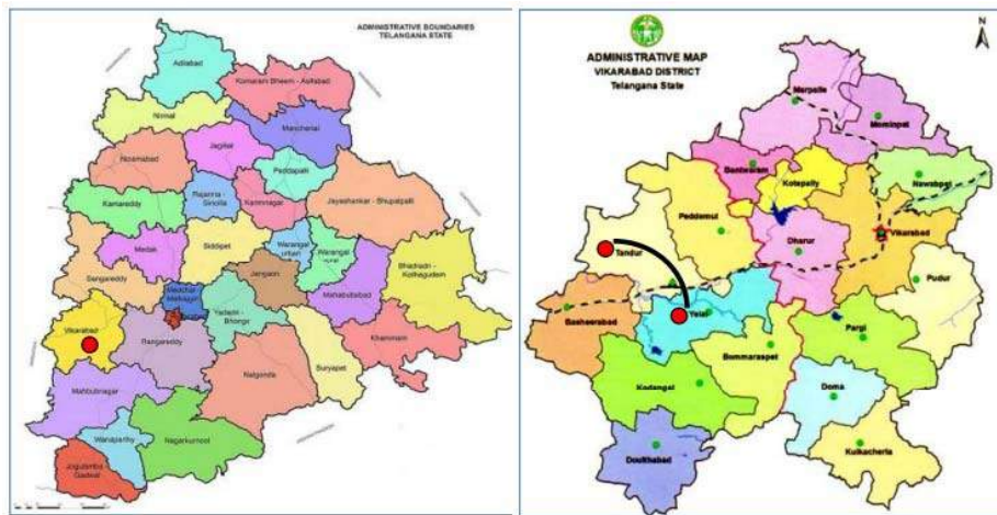
Fig. 1: Study area, Vikarabad district, Telangana
